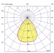
75° Optic
