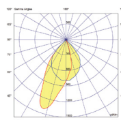
Wall Wash
